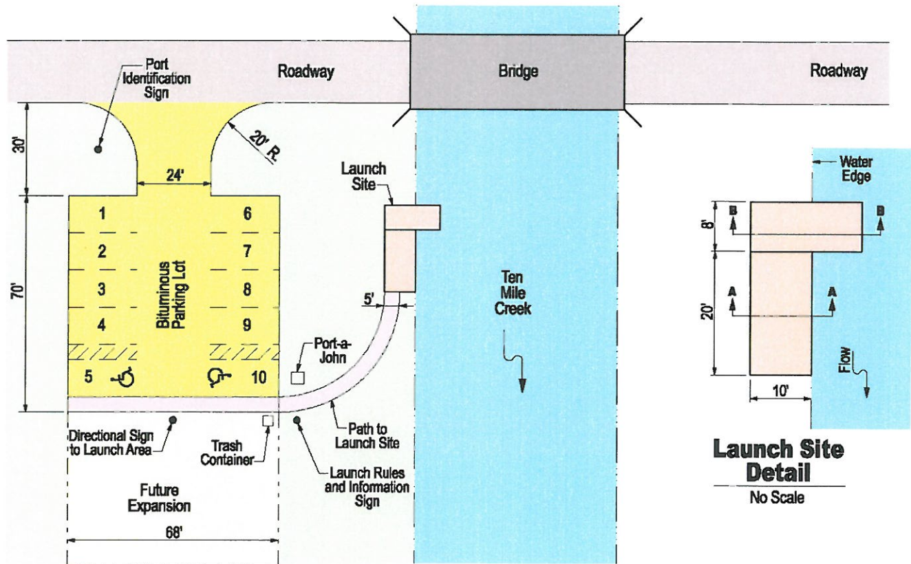
Typical Port Plan
